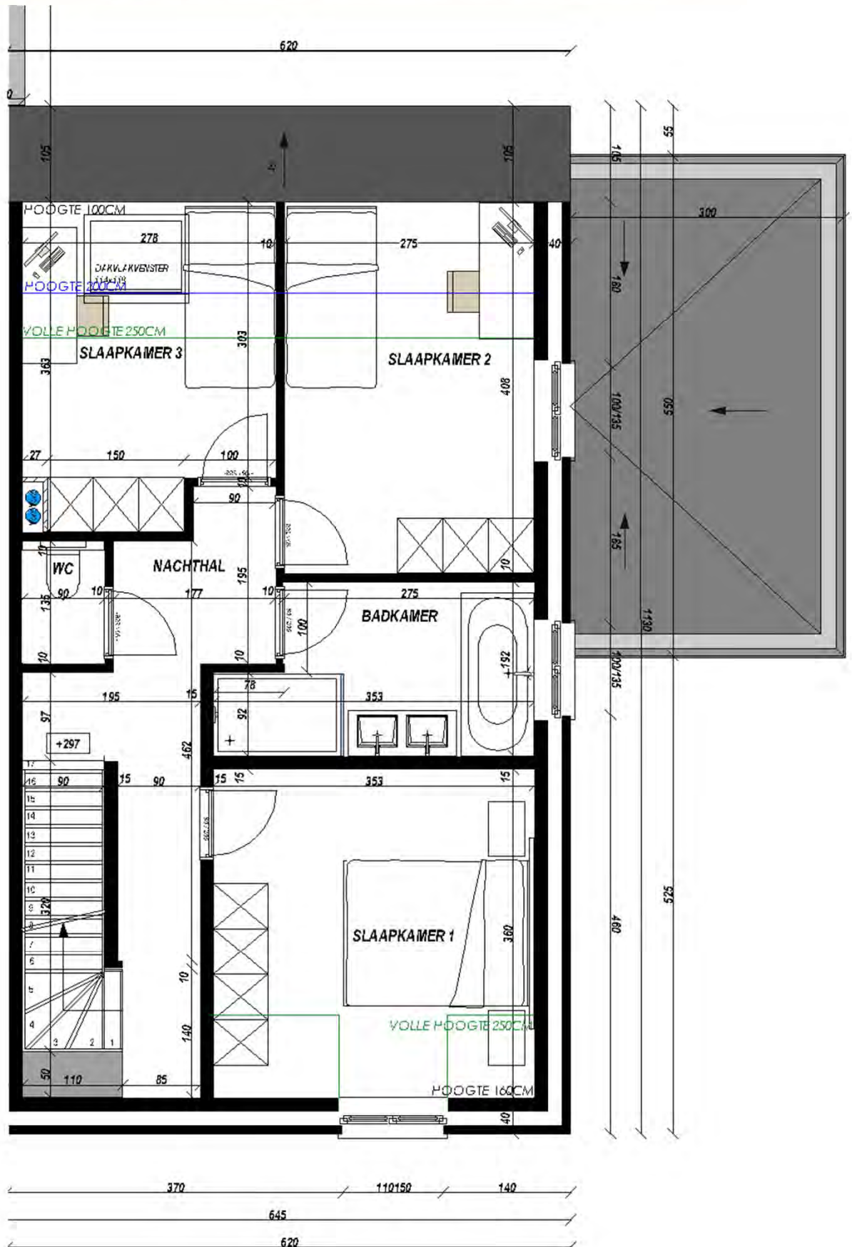
LOT 4 VERDIEPING 1 opp. : 63,61 m 2
