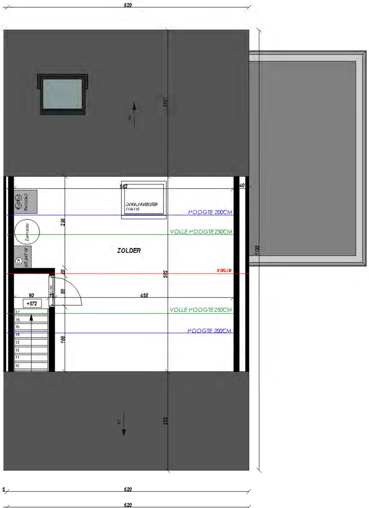
LOT 4 ZOLDER opp. : 31,12 m 2
